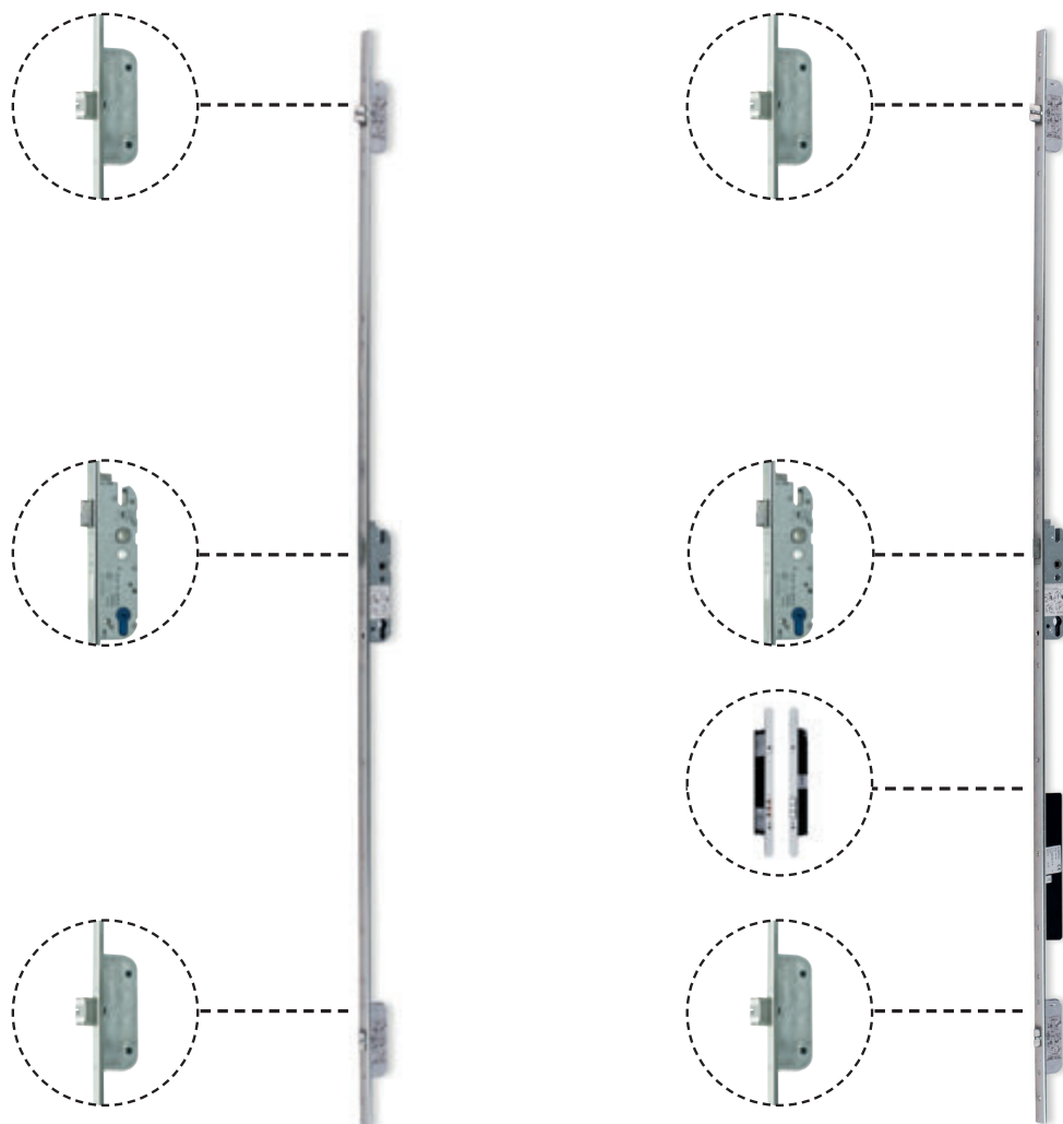
3 GU Automatic lock
